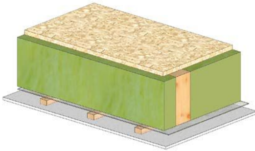
Internal ceiling construction 1 - in unheated room GIVE ESB A GO!
